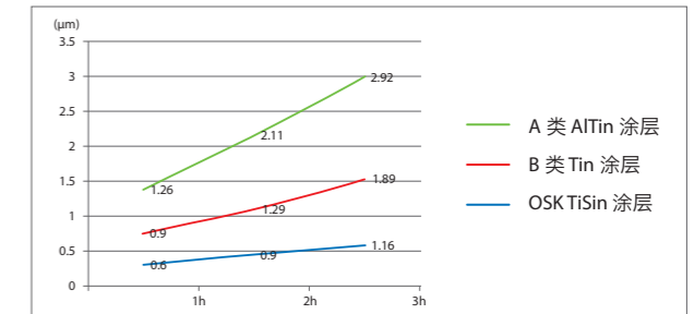
相同参数, 时间, 材料 (SKD11) 加工磨损涂层对比 The same parameters, time, material (SKD11) processing wear coating contrast
